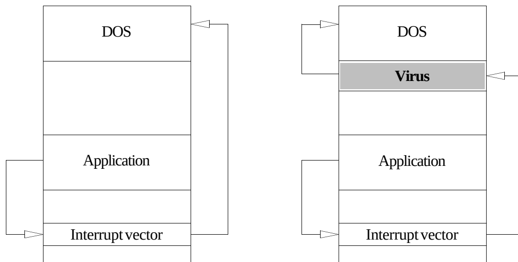
Figure 1. Interrupt routing before and after infection. INT 13 is a 'stealth' virus which uses interrupt interception to escape detection. MS-DOS applications use software interrupts to communicate with the operating system in a portable way. The jump addresses are stored in the interrupt table located at the beginning of memory. If a virus changes one or more of these addresses, any jumps to the operating system can be routed through the virus, which then decides what should be done with a particular request. The very first MS-DOS virus, Brain, employed interrupt interception. When active in memory, the virus intercepts any attempt to read from disk the contents of Sector 0 (the hiding place of Brain). The virus re-vectors such calls to point to the legitimate contents of Sector 0 which it has stored at a completely different location. Hence, when Brain is in memory, any attempt to look at the boot sector will not reveal its presence.
