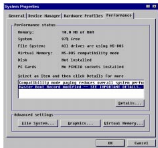
Figure 2: The messages in the system properties dialog in Windows 95 have been changed from previous versions.
