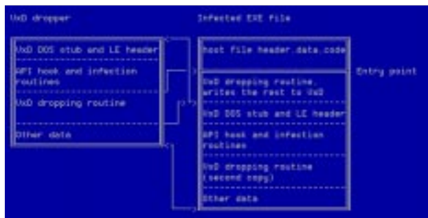
Figure 1: Punch exists in two forms; the VxD file version (found in VVFS.VXD ) and the EXE file version.
